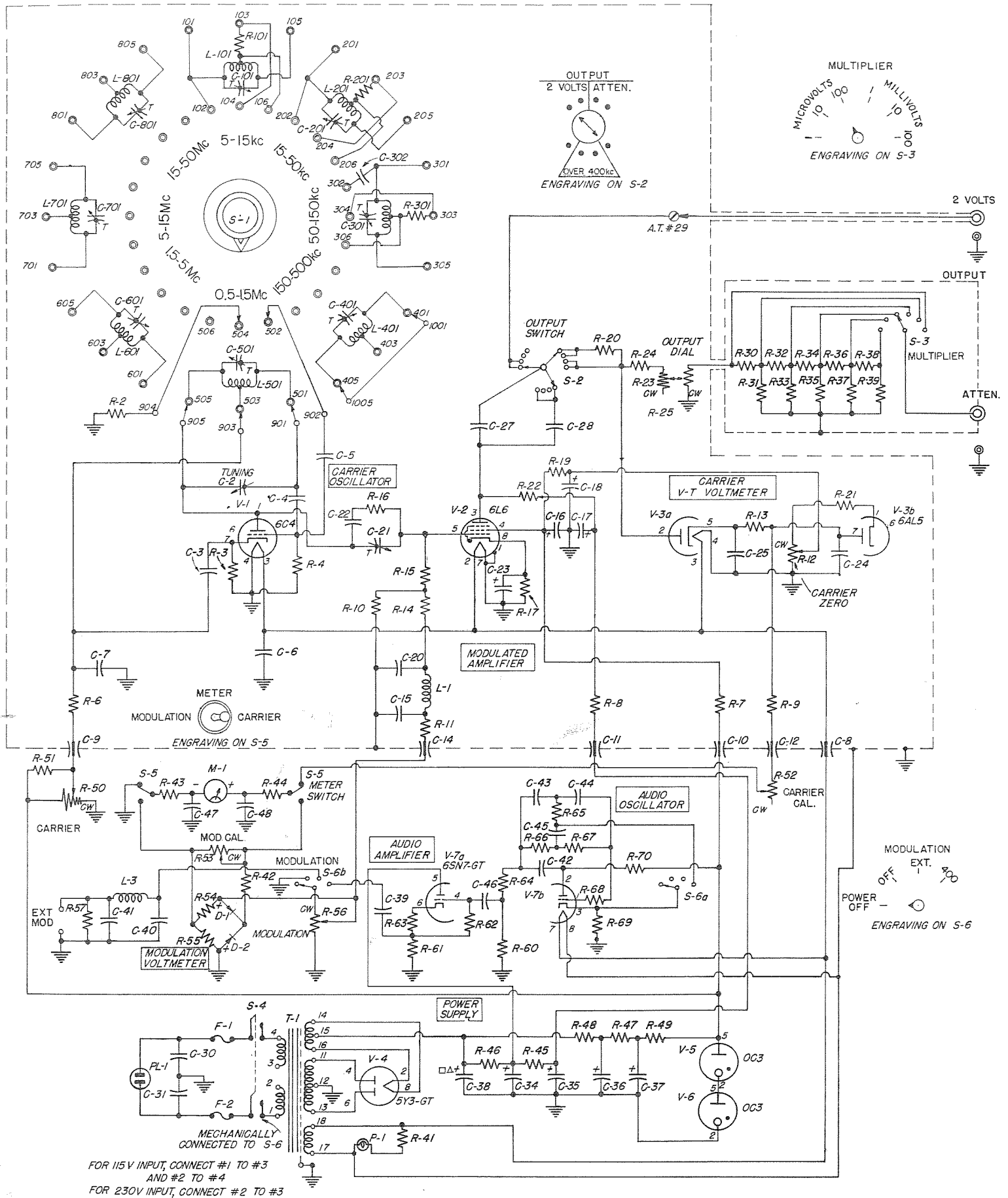
Figure 3. Wiring Diagram for Type 1001-A Standard Signal Generator
