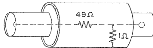
TYPE 1000-P3 VOLTAGE DIVIDER
